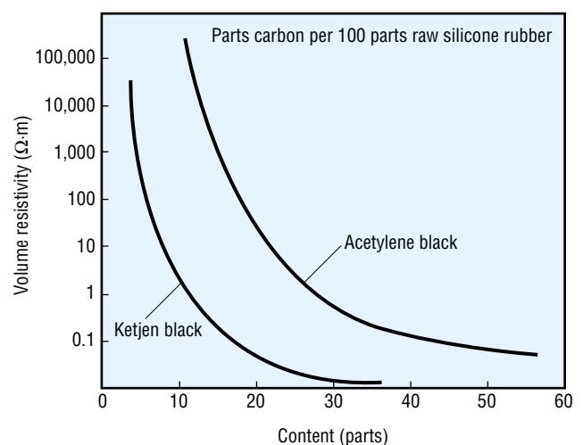
Volume resistivity and carbon black content
