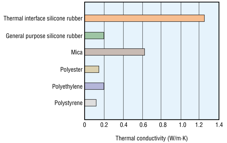
Thermal conductivity of thermal interface silicone rubber
